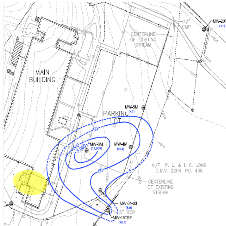
Upper Sandstone
