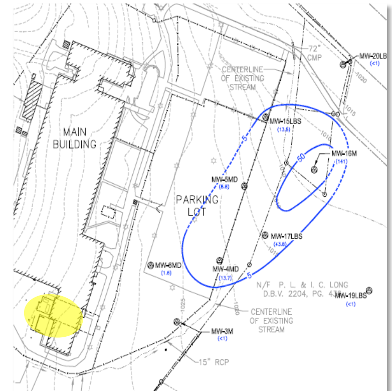
Lower Sandstone
