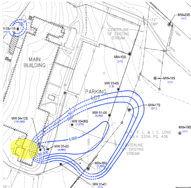
Marine Shale
