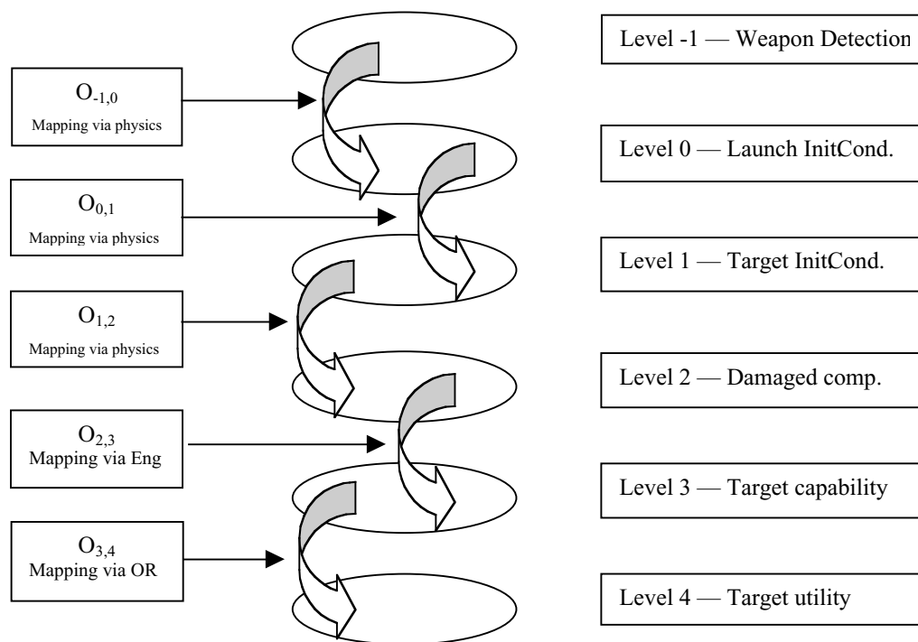
FIGURE 2—G GRAPHICAL DESCRIPTION OF THE MATHEMATICAL SPACES AND OPERATORS [GONZALEZ ET AL., 2000]
