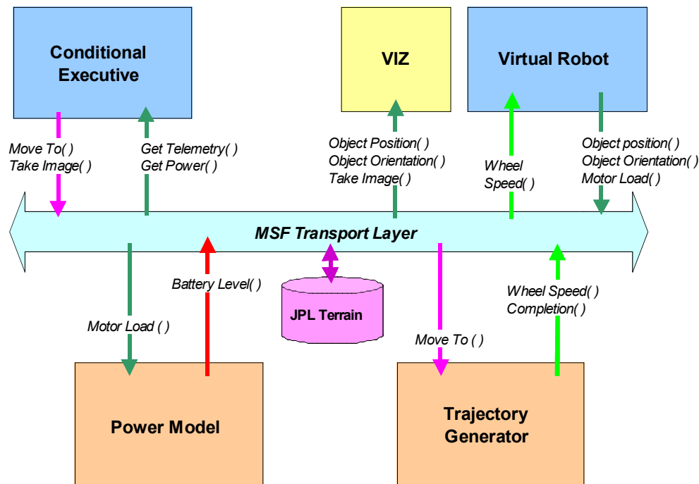
Figure 3. Components and messages of the June 2002 MST release.
