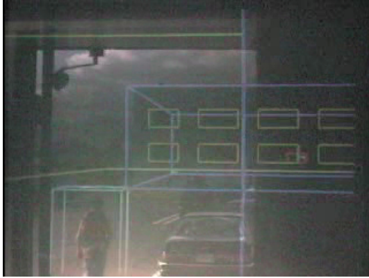
Figure 1: A remote BARS user is highlighted with a box shape. In this example, the user is also physically visible, but the position information is transmitted for all mobile users and can show the location of an occluded user.
