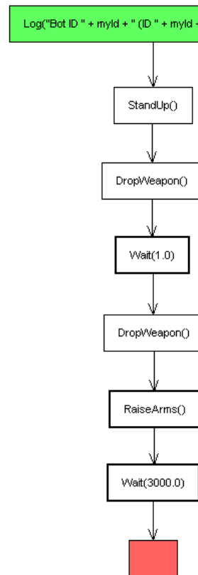
Figure 4. The Surrender Behavior
