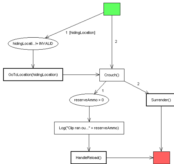
Figure 3. The ClipEmpty Behavior
