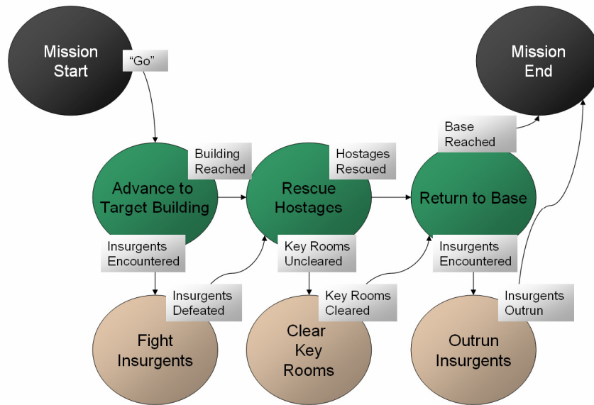
Figure 2. Simplified FSM of a hostage rescue mission.
