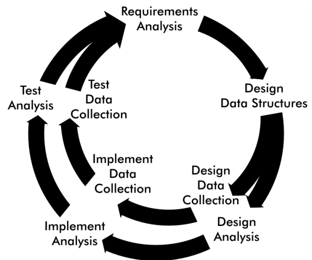
Figure 3. Agile Methodology
