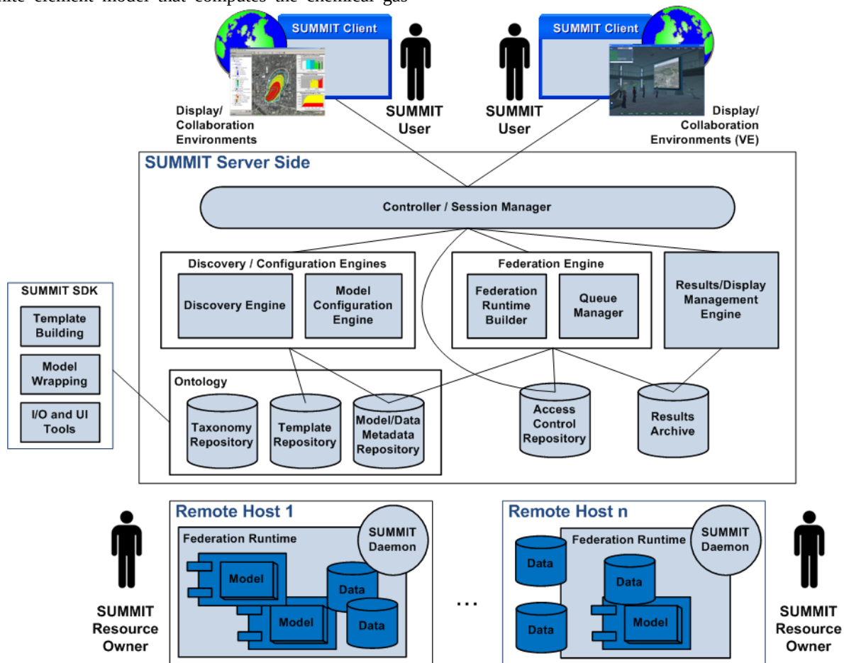
Figure 1. SUMMIT Architecture
