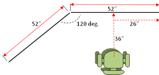
Figure 4. Layout of Simulator Screen and Subject Positioning
