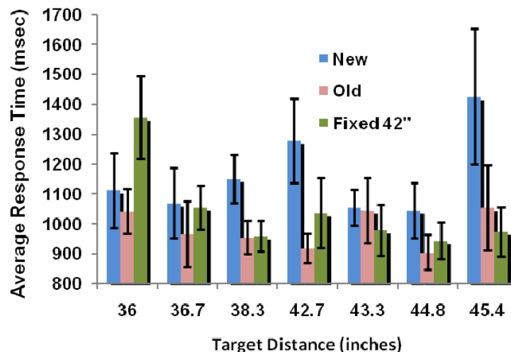
Figure 13. Response Time as a Function of Target Position and Vergence Condition
