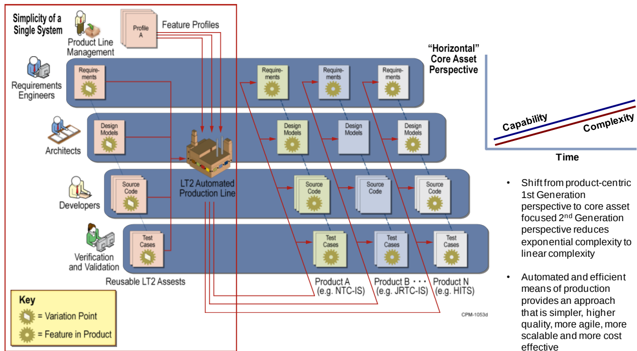
Figure 3: Efficiency of 2nd Generation SPL Approach
