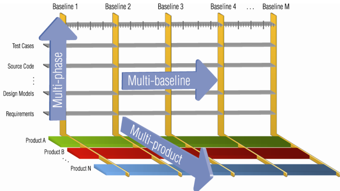
Figure 4: Synchronous concerns of an SPL solution
