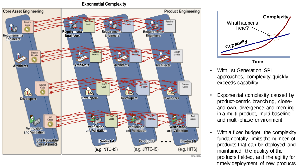
Figure 2: Complex interdependencies resulting from the product-centric perspective
