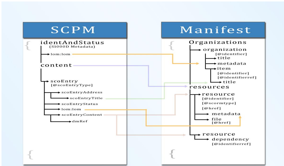
Figure 2: SCPM Mapped to the IMS Manifest
