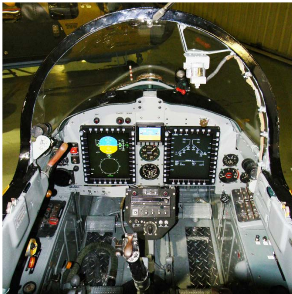
Figure 2. Trainer cockpit with MFDs Installed
