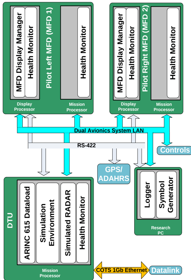
Figure 1. System Architecture
