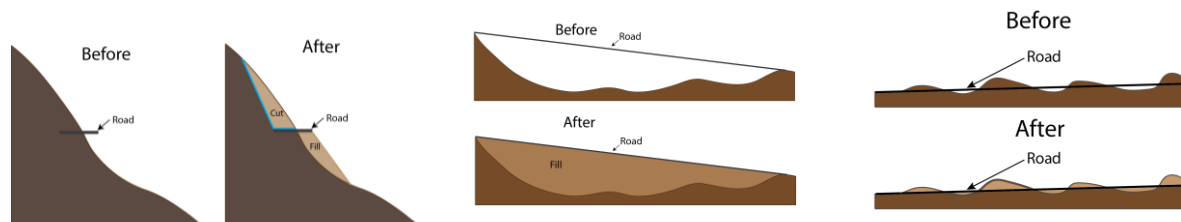
Figure 3 - Cut and Fill Operations (Left: Side Slope, Middle: Forward Slope, Right: Undulation Removal)
