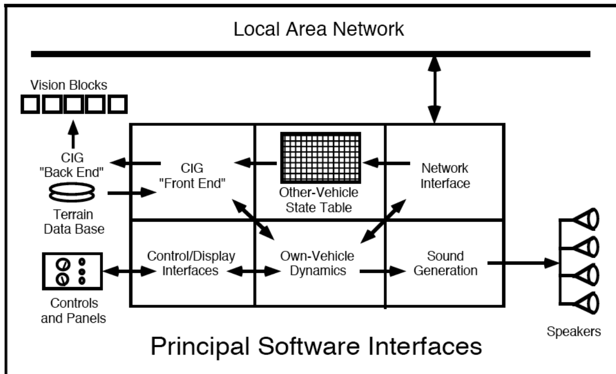
Figure 1: Principal software interfaces for a typical simulator
